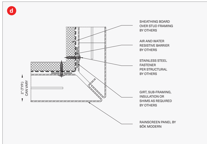
MITERED CORNER
