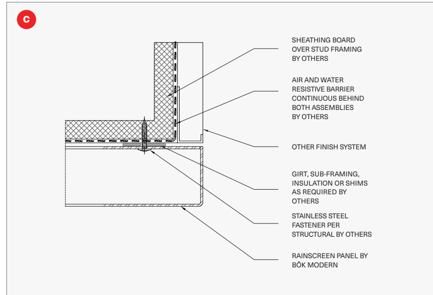
END CONDITION
