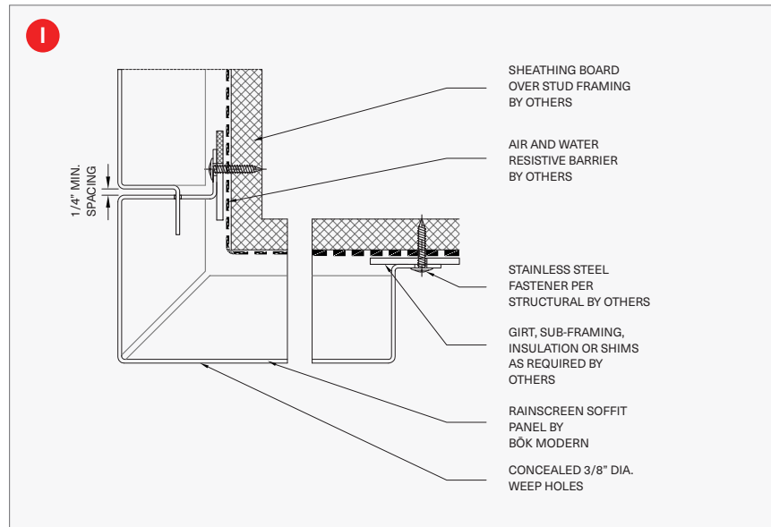
SOFFIT CONDITION
