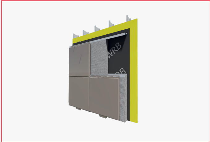
Z CHANNEL OVER EXTERIOR BATT INSTALLATION
