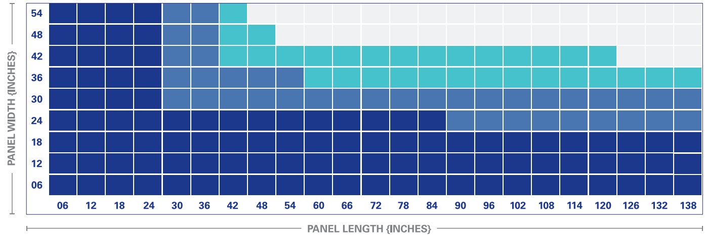
BOK MODERN ALUMINUM PRE-ENGINEERED RAINSCREEN PANEL DESIGN TABLES Based on maximum wind loading (psf) DEFLECTION CRITERIA All loading based on L/60
